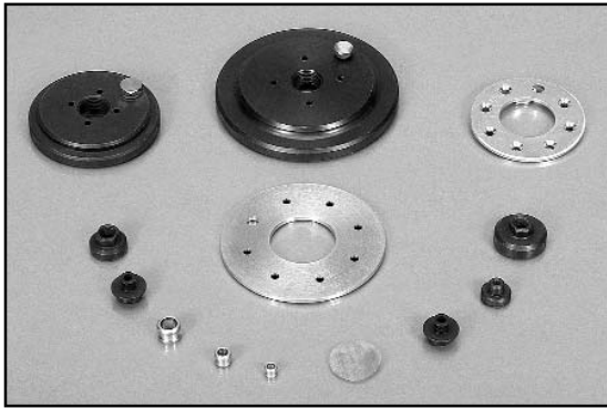
ANVER Generic Replacements of P-Style Vacuum Cups and Suction Cups Fittings
