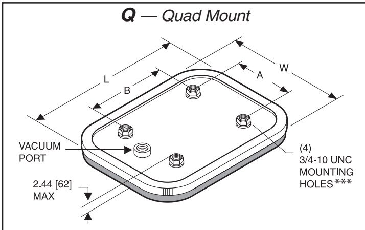
*** FP070200Q-A2B7 supplied with M10-1.5 metric threads
